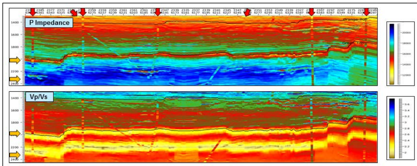
Figure 1: Typical inversion of the Gulf of Mexico data. P Impedance and Vp/Vs are shown overlain by high-cut filtered logs. The constant trend model hung on structure, modified by interval velocities and augmented by facies-based trend values (see text) was used. The two wells on the right side of the figure disagree with the inversion in a low frequency sense. Testing demonstrated that they were indeed outliers in this respect.
