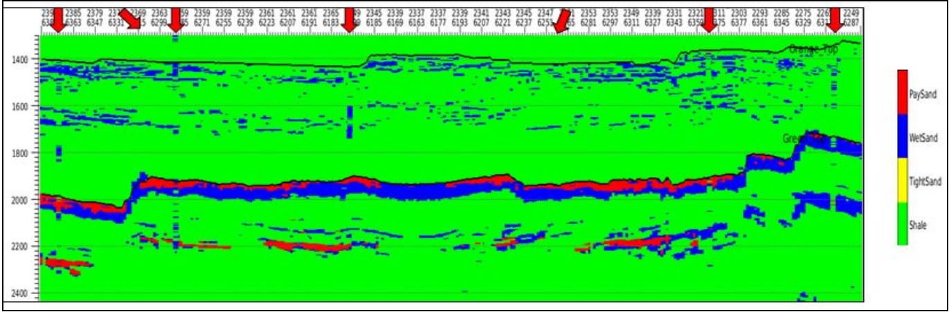
Figure 5: Information from processing interval velocities and facies trends have been added as described in the text. Agreement with the wells has improved and there is an indication of an oil-water contact.
