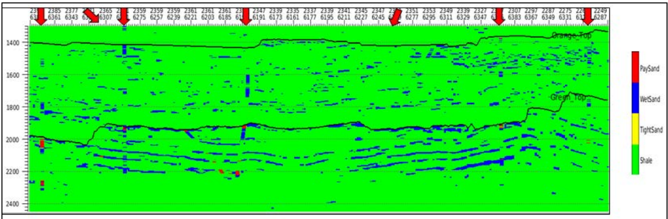
Figure 3: Bayesian classification from an inversion which used very simple non-facies based trends as an input low frequency model. The imprint information of the pay sands in the low frequency band is missing and the result shows no sand fairway and no pay.
