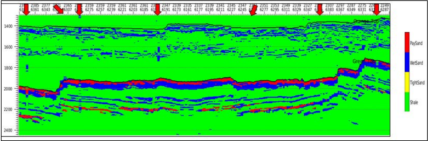
Figure 4: Here frequencies describing the imprint of the sandstones in the low frequency band have been added to the low frequency model for the inversion. These are laterally-invariant and hung on structure. They are best-fit to all the logs. Sand facies have now been identified which correlate to the petrophysical facies in the logs.
